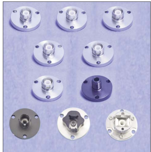
Bulkhead receptacles for ultra, super, or angled connectors with or without stoppers
