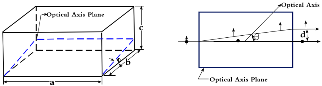
YVO 4 Beam Displacer for Circulator
