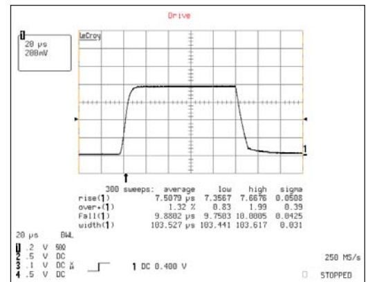
Current Pulse in QCW mode at 80A Output with the LDX-36040-70
