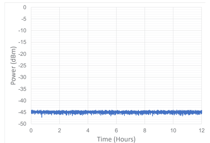
Carrier suppression stability
