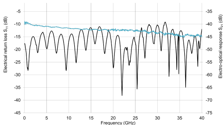
Typical Curve S_{21} & S_{11} from RF 2 Electrode
