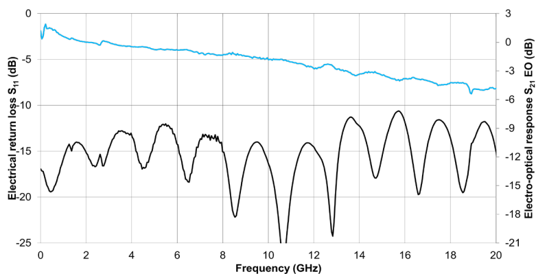
Typical Curve S_{21} & S_{11} from RF 1 Electrode
