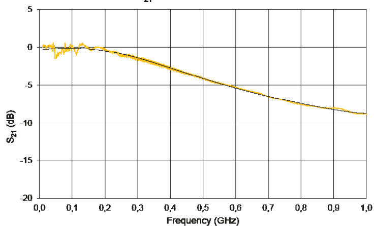
MX-LN-0.1 Typical S_{21} Curve
