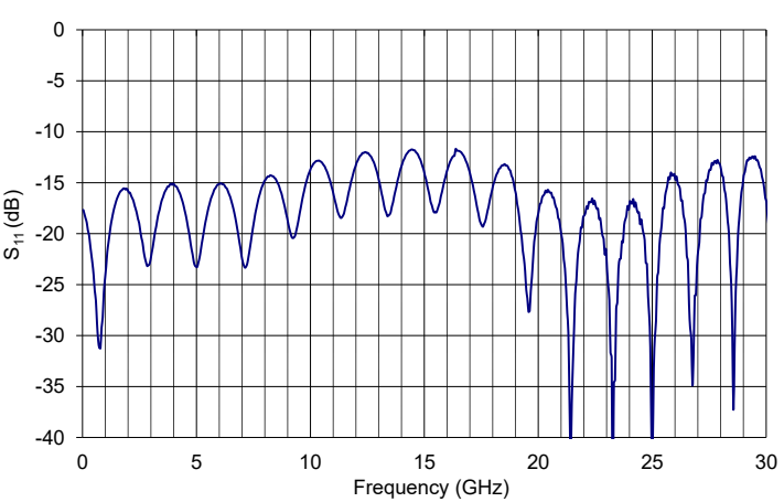
MX-LN-20 Typical S_{11} Curve
