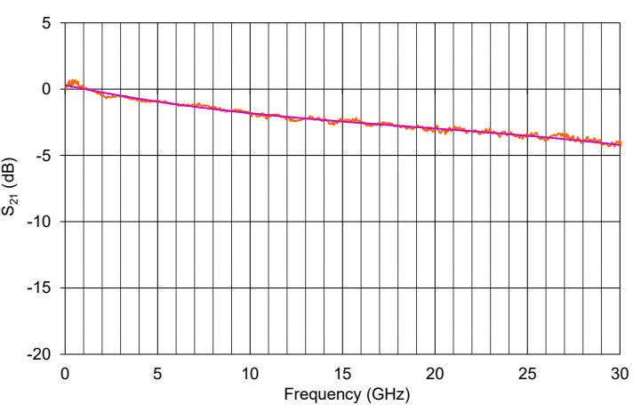
MX-LN-20 Typical S_{21} Curve
