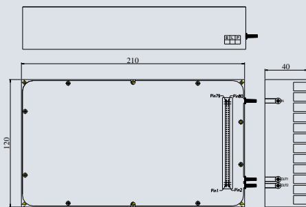
Mechanical Dimension (210 X 120 X 40mm)
