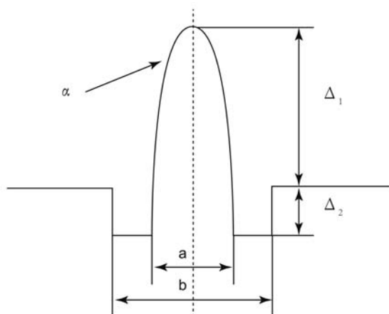
The refractive index profile sketch
