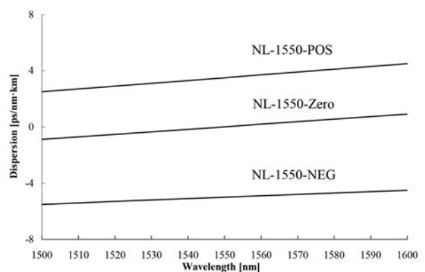
Three types of HNLf typical dispersion test curve
