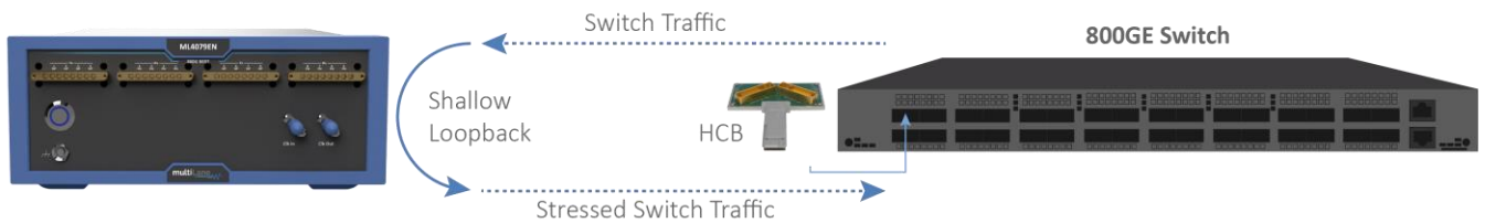
Figure 13: Shallow Loopback using ML4079EN and 800G switch
