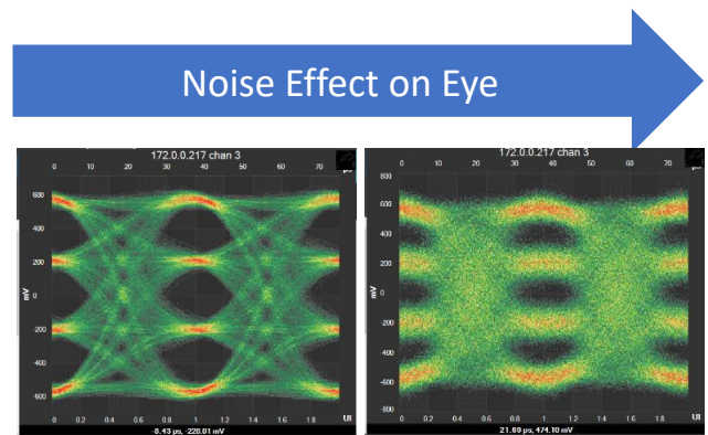
Figure 12: Eye Diagram before and after noise injection – PAM4 modulation
