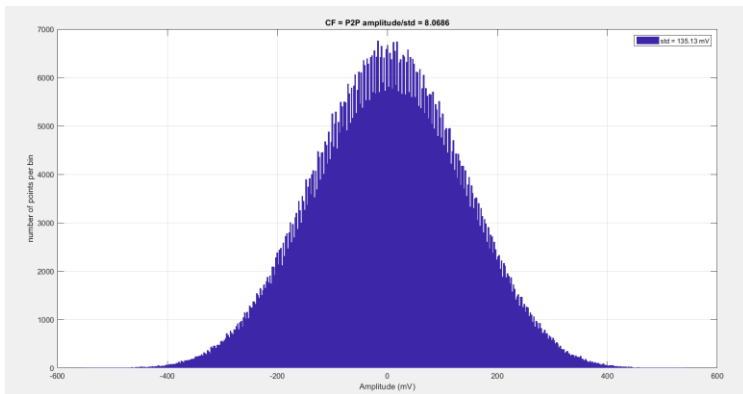
Figure 8: Crest Factor Measurement: Gaussian Noise
