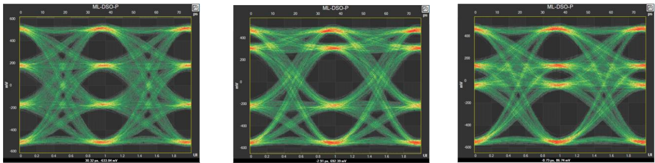
Figure 14: Inner/Outer Eye Control using ML4079EN
