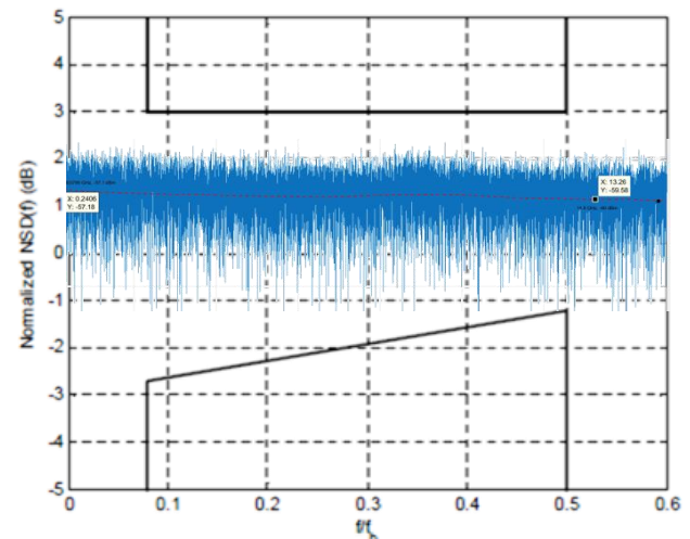
Figure 9: Noise Flatness
