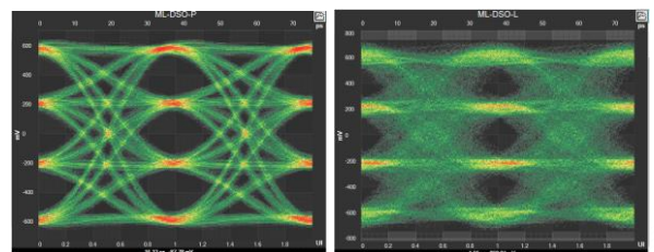
Figure 5: Jitter Measurements
