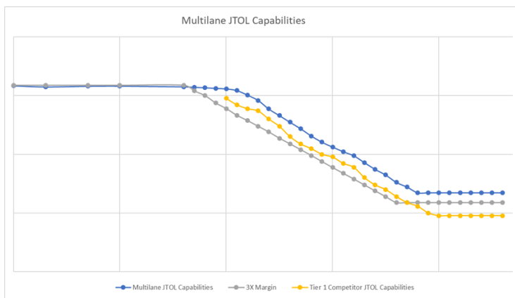
Figure 4: MultiLane Capability vs IEEE Mask
