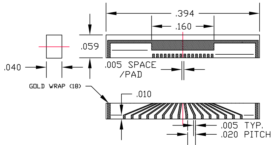
CERAMIC 16 ELEMENT ARRAY A14577
