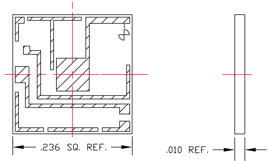
SQUARE CERAMIC A14451
