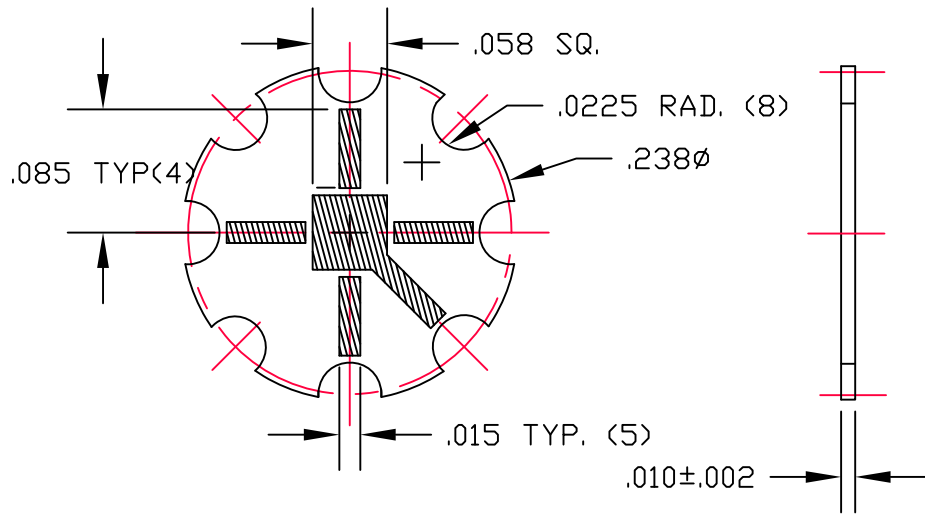
QUAD HEADER A14084
