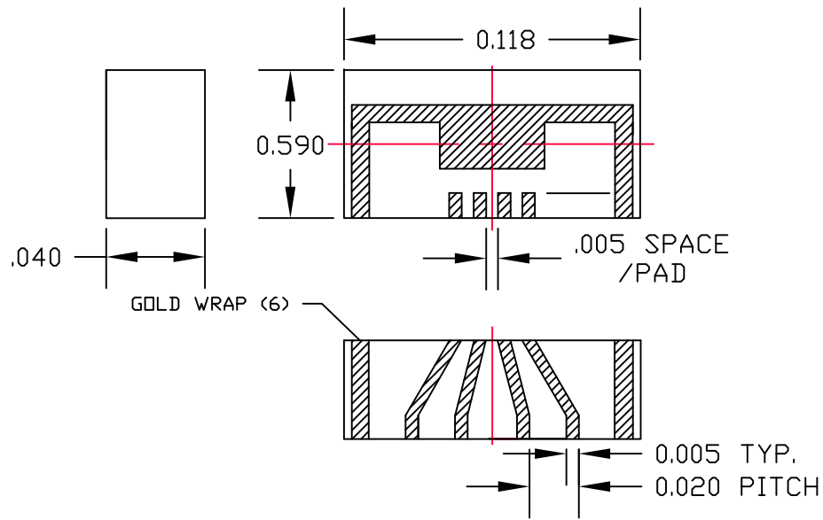
CERAMIC 4 ELEMENT ARRAY A14536
