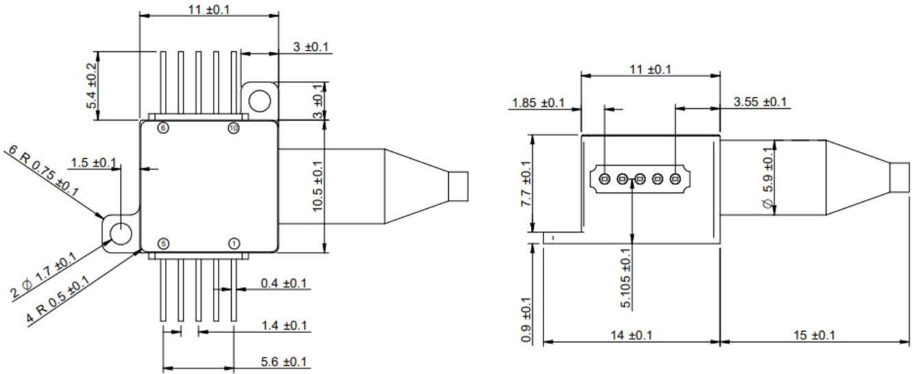
Figure 1. Mechanical Dimension
