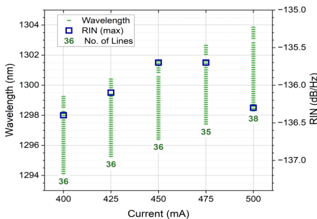
Individual Mode RIN
