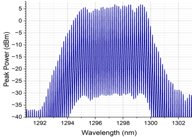
Optical Spectrum (res. 10pm)
