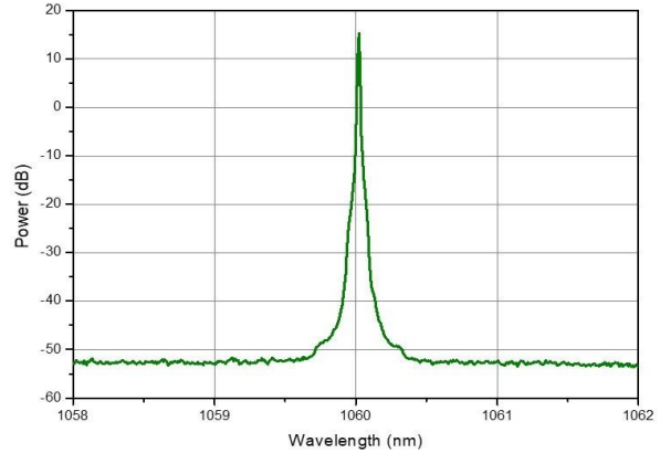
Optical spectrum @ 600mA (res. 20pm)
