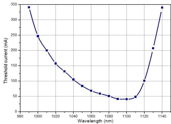
Threshold current
