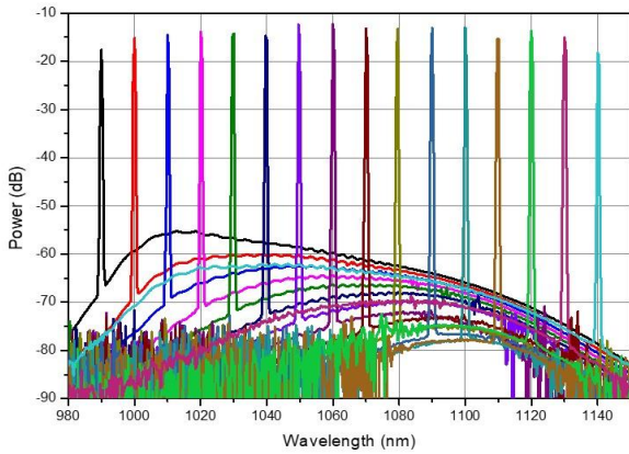
Optical spectra @ 600mA (res. 100pm)
