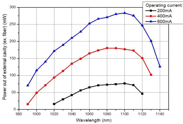
Output power spectra
