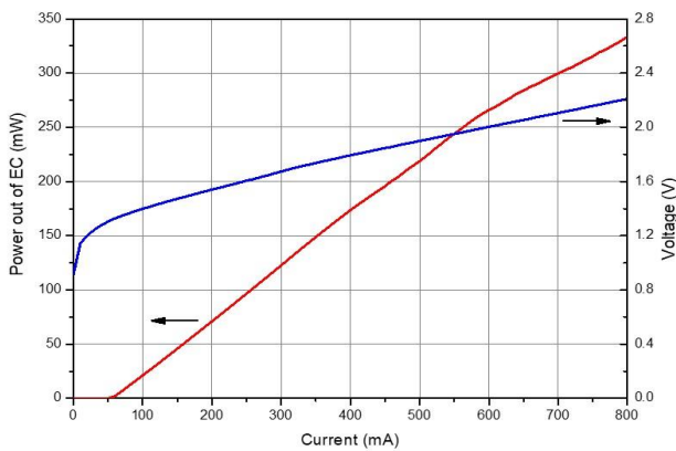
Output power @ 1100nm
