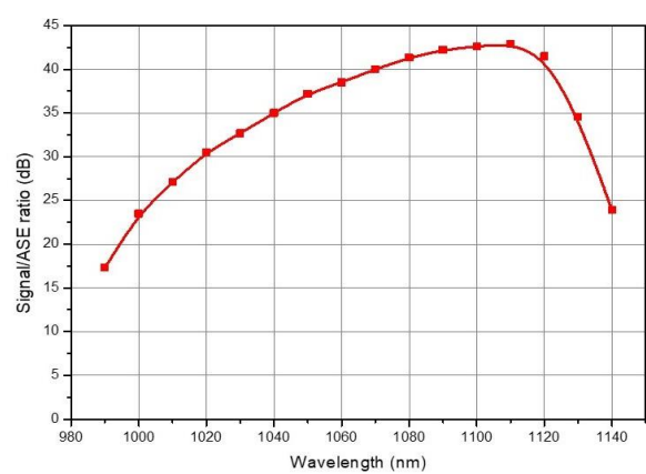
Integrated Signal/ASE ratio @ 600mA
