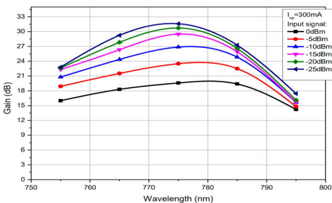
Gain spectra at different input signals
