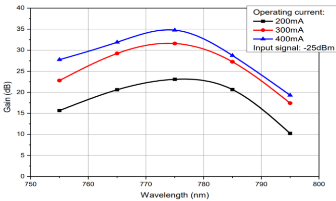
Gain spectra at different currents
