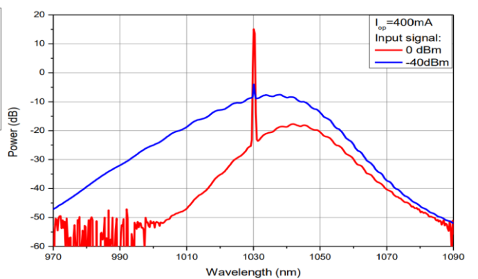
Spectra of amplified optical signal
