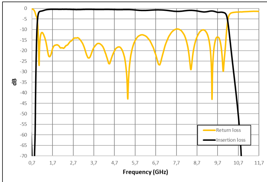
Figure 1: ERZ-BPF-0110-1000-2 Insertion & Return loss
