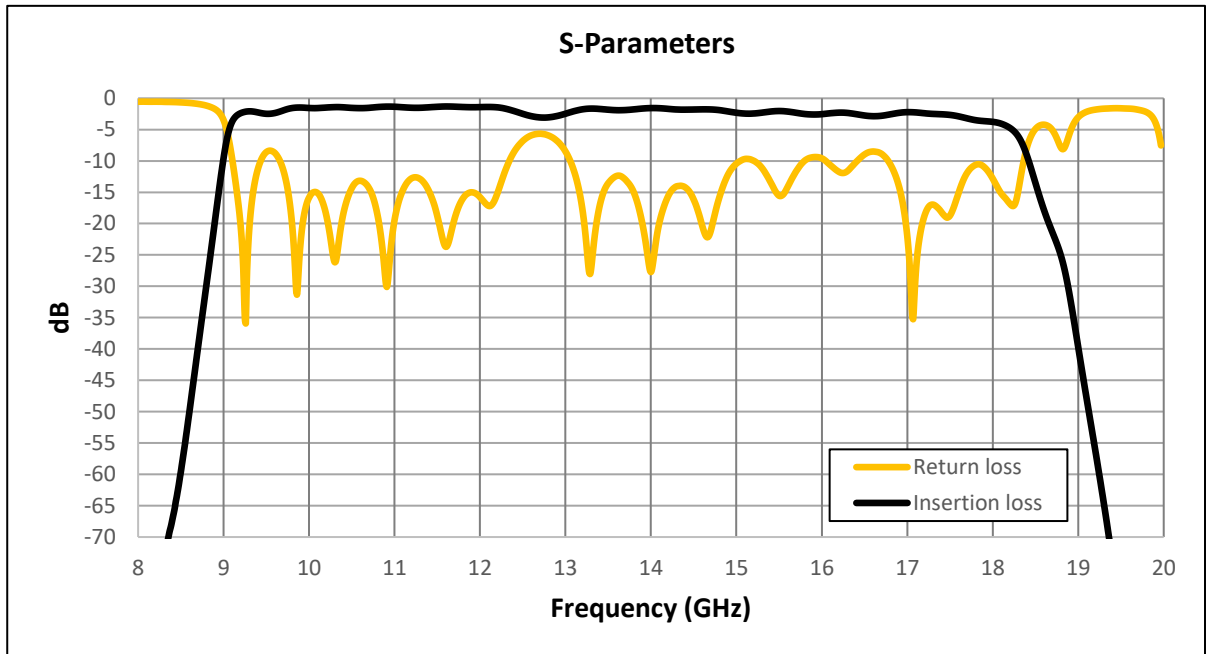
Figure 1:ERZ-BPF-0920-1800-3.7 Insertion & Return loss
