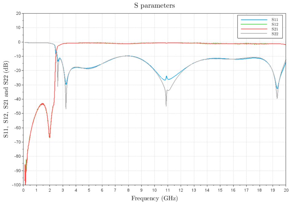
Figure 1: ERZ-HPF-0280-1800-1.5 Insertion & Return loss
