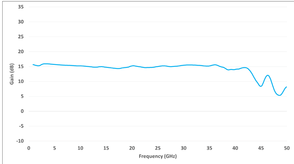
Figure 1: HL5887 Gain (opt. -29-JJ)
