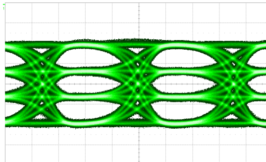
Fig. 7: 56 Gbps PAM4 pattern on RF In, 100mV/div.
