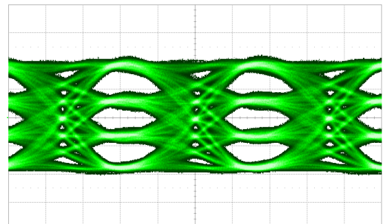
Fig. 8: 56 Gbps PAM4 pattern on RF Out, 600mV/div.
