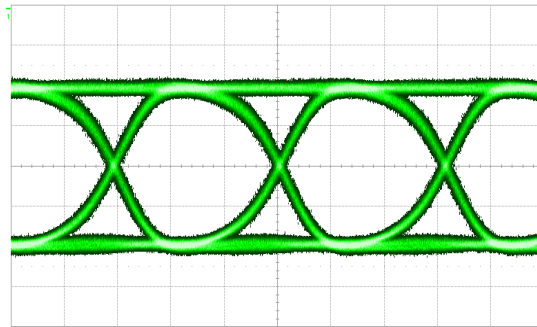
Fig. 5: 32 Gbps PRBS11 pattern on RF In, 100mV/div.
