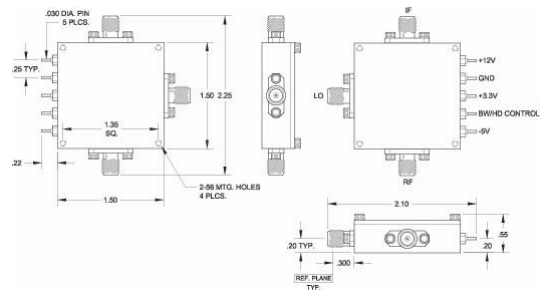
Figure 2: Dimensional Drawing of the HL9313
