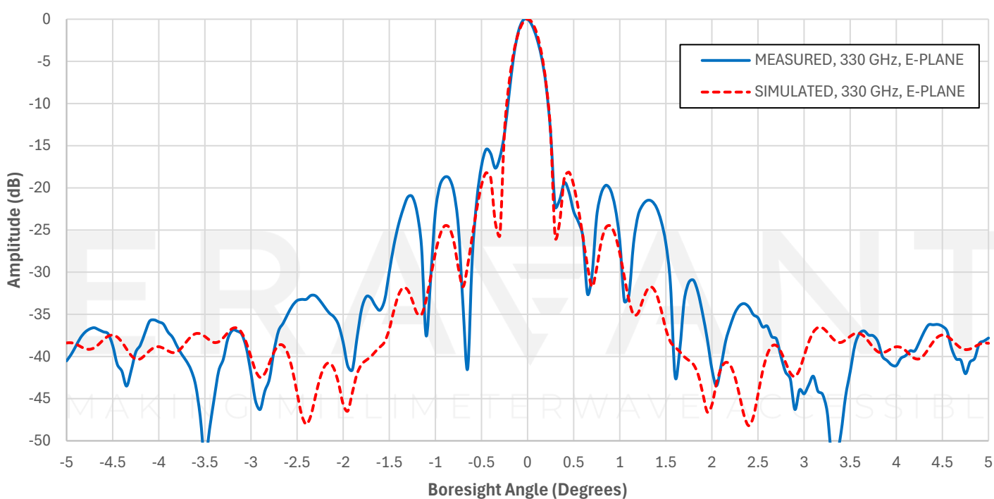
SAY-224334503-03-S1, E-Plane Measured vs Simulated Pattern, 330 GHz
