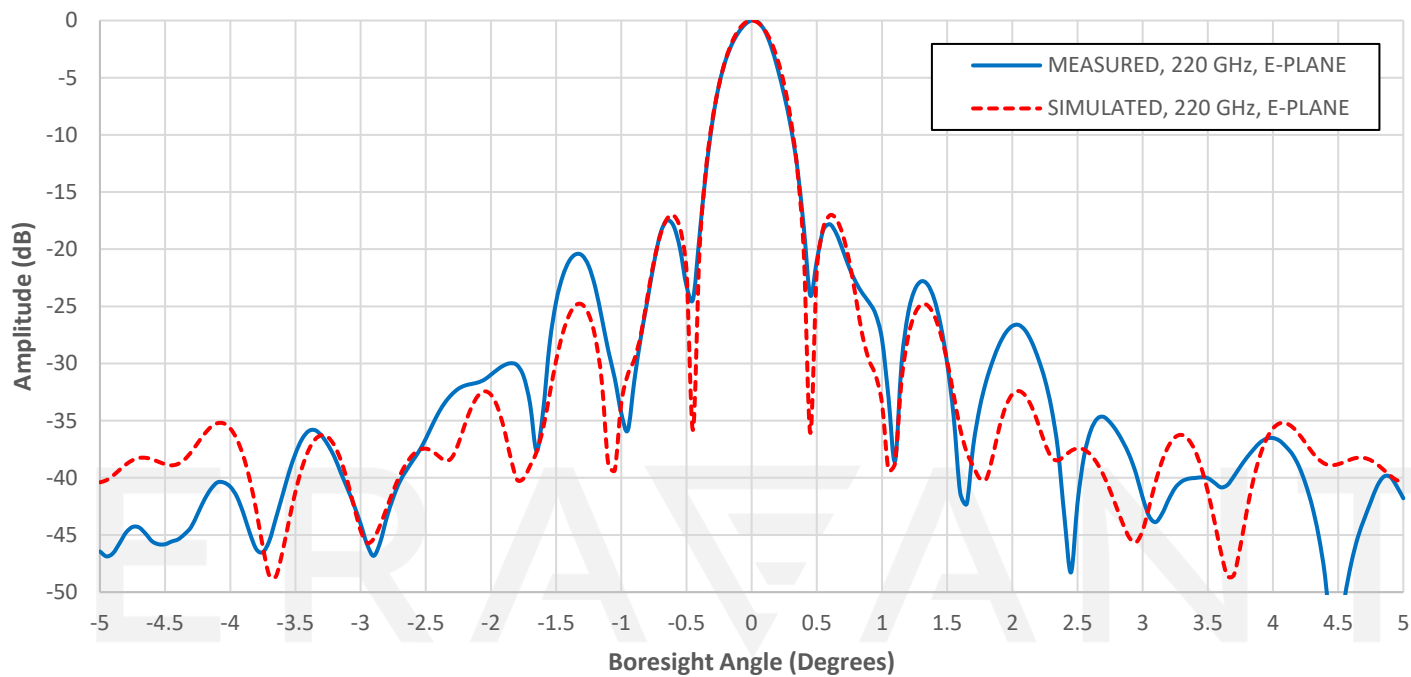
SAY-224334503-03-S1, E-Plane Measured vs Simulated Pattern, 220 GHz
