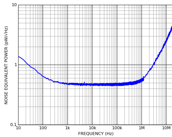
PD10B-80-DC (80 kV/A) noise equivalent power
