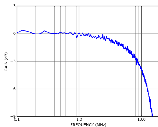
PDX10B-80-DC-SI (80 kV/A) frequency response
