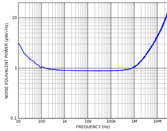
PDX10B-80-DC-SI (80 kV/A) noise equivalent power
