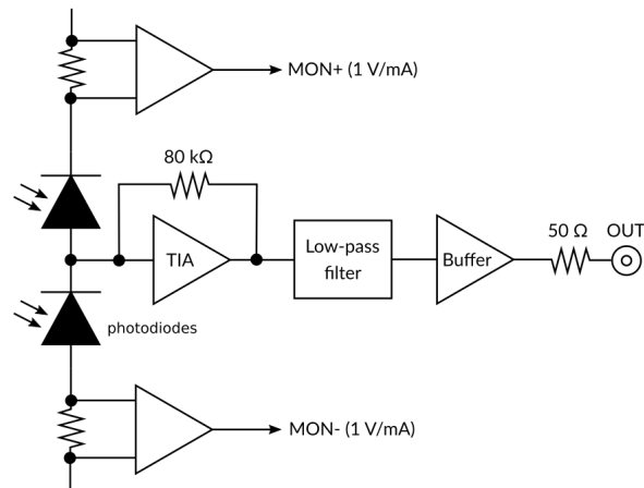
PDX10B-80-DC-SI functional diagram
