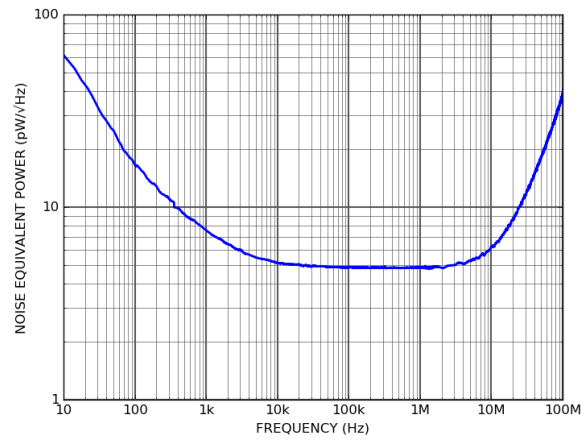
PDX10B-3-DC-SI (3 kV/A) noise equivalent power
