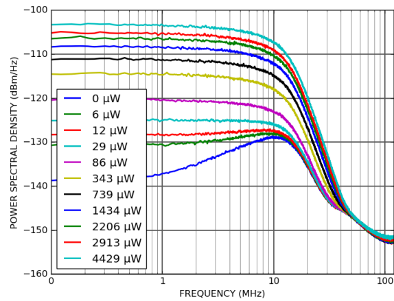
PDX10B-80-DC-SI (80 kV/A) output power spectral density
