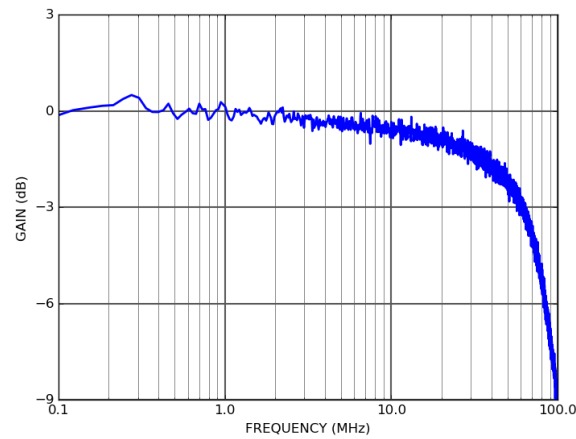
PDX10B-3-DC-SI (3 kV/A) frequency response
