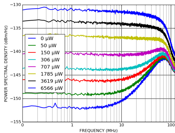
PDX10B-3-DC-SI (3 kV/A) output power spectral density
