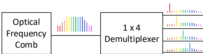
The iCLA is a monolithic InP PIC combining a comb laser with a demultiplexer to deliver 4 coherent wavelengths on individual fibers for modulation
