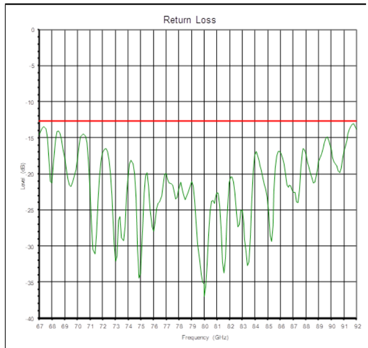
Typical Return Loss for Model 26810-QA 50mm Diameter Antenna
