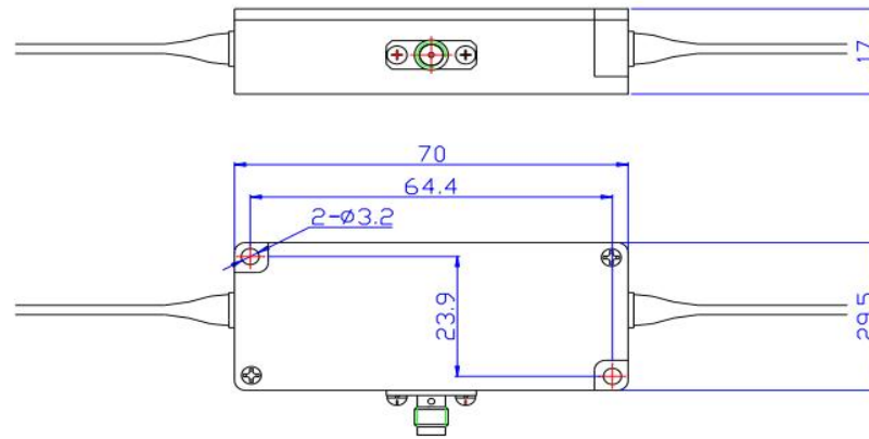
Package FA
